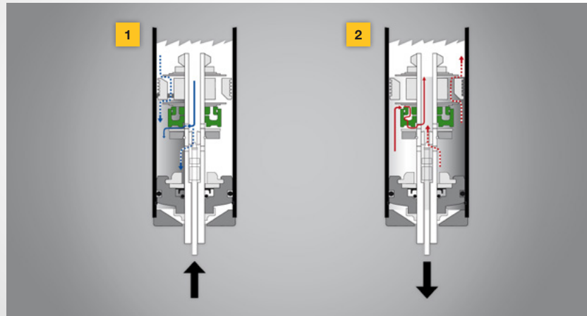
Figure 1: (Compression flow) At low shaft speeds, oil flows mostly through the shaft jet bleed (lower dotted arrow). At higher shaft speeds, oil flows mostly through the compression ports in the piston (upper dotted arrow). At very high shaft speeds, or during sudden shaft accelerations, oil can also escape through the compression ports in the DFV, increasing comfort.
