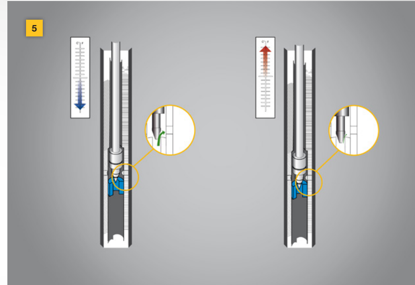
Figure 5: Thermal Expansion
